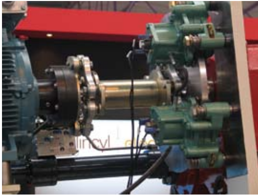
Ixilflex® with torque limiter.
