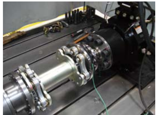
Ixilflex® on test bench.
